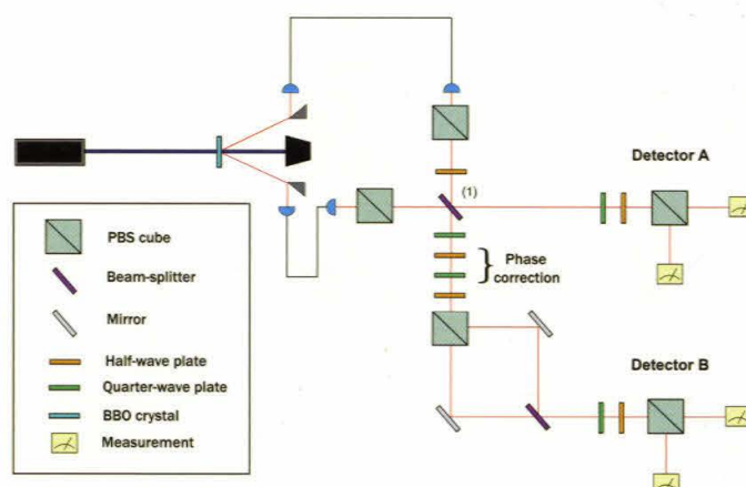
Figure 4: Circuit for generating and manipulating the quantum cluster state.
