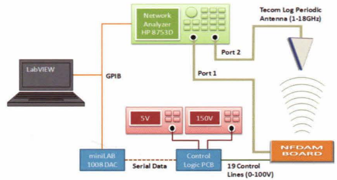
> Figure 5: Measurement Setup Block Diagram
