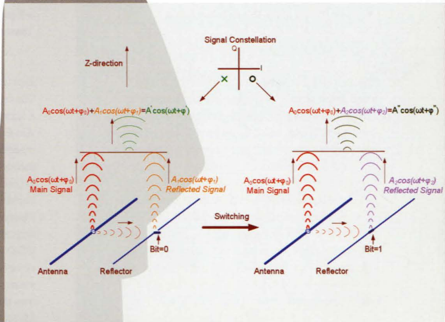
Figure 3: Signal modulation using switches on the reflectors.
