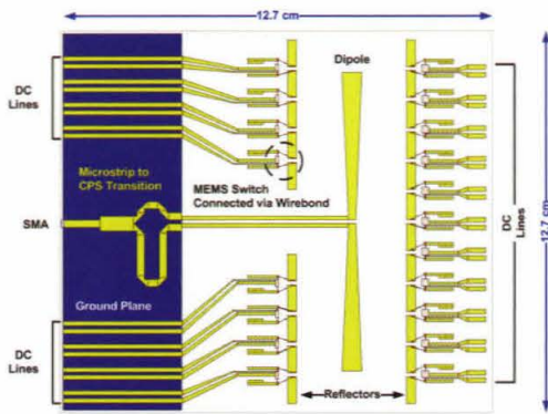
> Figure 4: Layout of the fabricated 2.4GHz NFDAM transmitter on microstrip.
