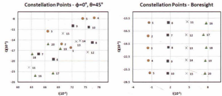
> Figure 7: Measured constellation points of the NDFAM Transmitter microstrip.
