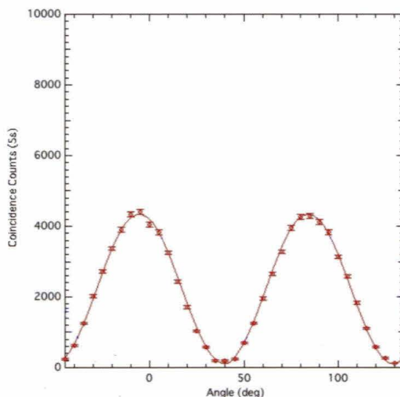
Figure 7: Detail of the manipulation of the state of the path qubit via polarization qubit measurements.
