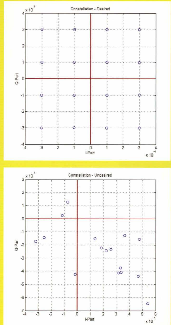
> Figure 2: Simulation of 16QAM in desired direction (top) and undesired direction (bottom). Blue circles represent symbols.
