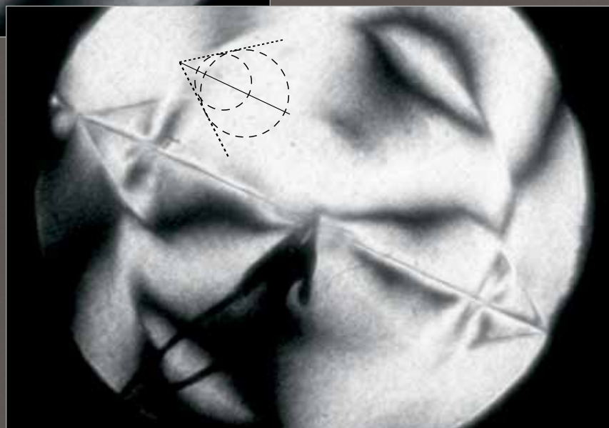
Above: Earthquakes generated in the laboratory illustrating the transition from Sub-Rayleigh to supershear rapture speeds. Right: Note the creation of the shear wave mach cones in the solid.
